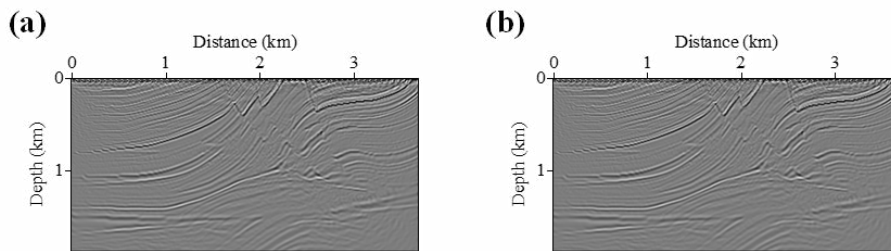
Figure 10 The reverse time migration of Marmousi TTI model.
