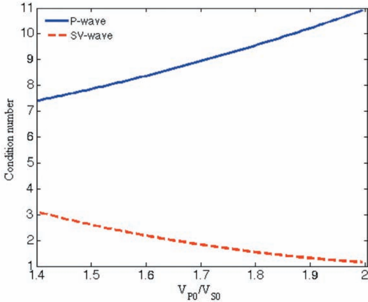
Fig. 2. Condition number calculated as a function of the V_{p0}/V_{s0} ratio for P-waves from eq. (9) and SV-waves from eq. (10).
