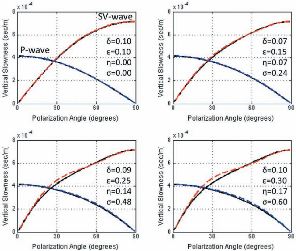
Fig. 1. Exact vertical slowness ( q ) as a function of the polarization angle ( \psi ) for P- and SV-waves (solid curves) and the corresponding weak-anisotropy approximations computed from eqs. (9) and (11) (dashed curves). The plots correspond to four VTI models with V_{P0} = 2420 m/s and V_{S0} = 1400 m/s (the models are taken from Tsvankin, 2012).
