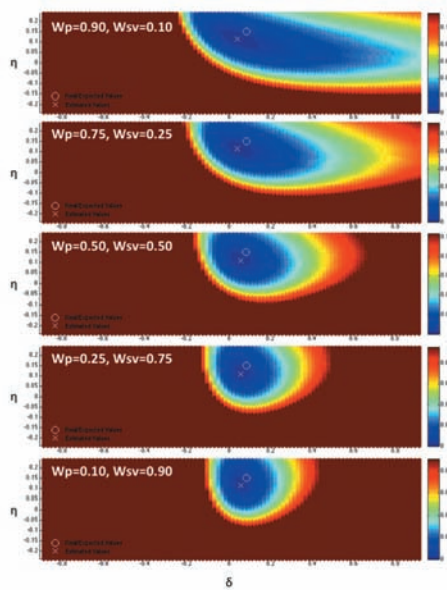
Fig. 10. Summary of estimation errors in \delta and \eta for different W_p and W_{sv} combinations in the entire VSP interval.
