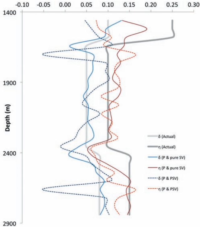
Fig. 12. Polarization angles of pure SV- and converted PSV-waves used in the joint inversion.
