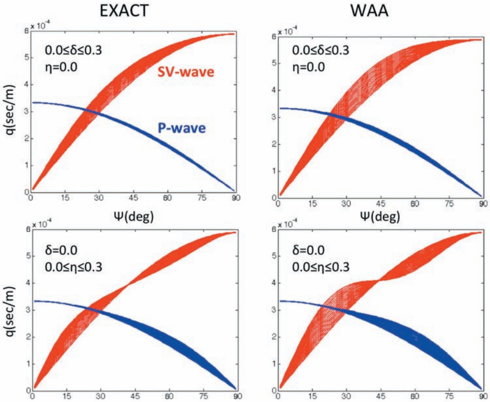
Fig. 3. Relationship between the vertical slownesses and polarization angles of P- and SV-waves for a range of \delta - and \eta -values ( V_{p0}/V_{s0} = 1.76 ). The curves on the left plots are computed from the exact equations and on the right plots from the weak-anisotropy approximations.
